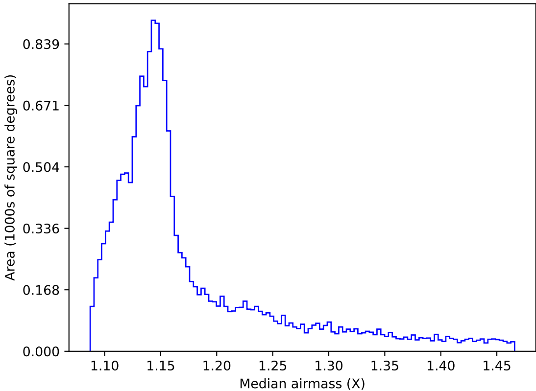
weather_cloudso1v3.4_10yrs WFD all bands: Median airmass
