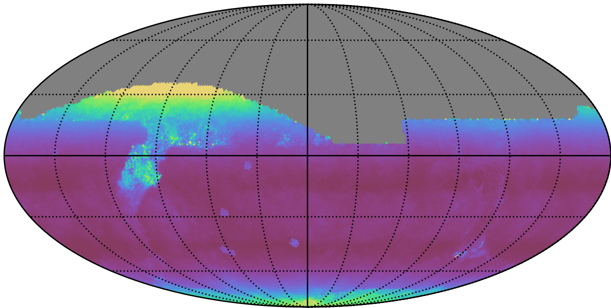
weather_cloudso1v3.4_10yrs All sky z band: Median airmass
