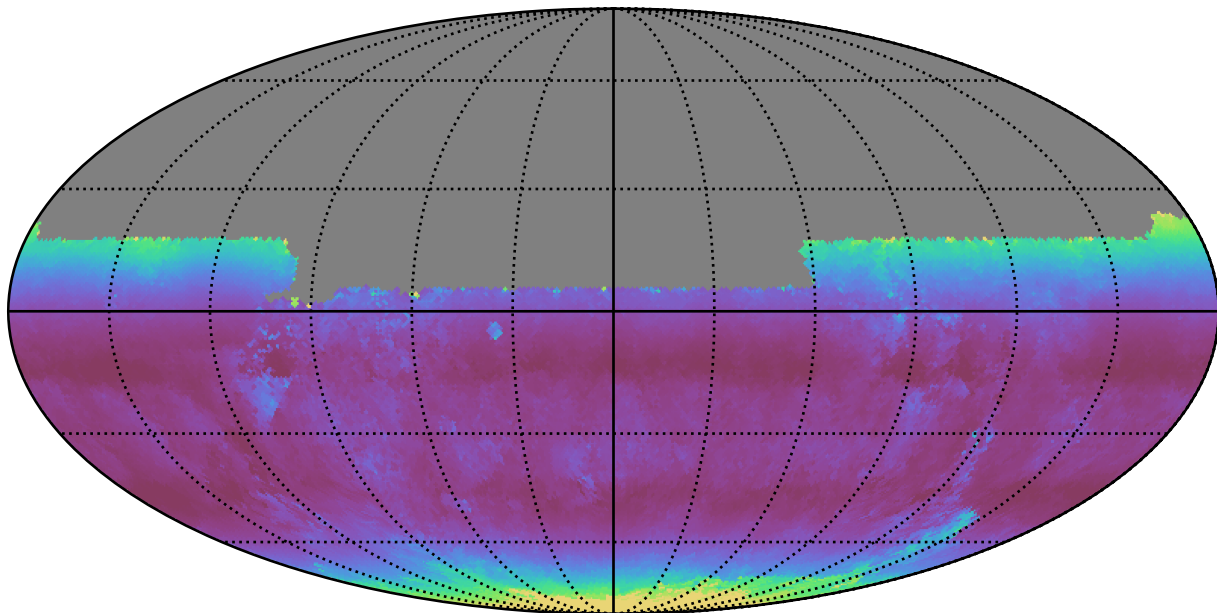
weather_cloudso1v3.4_10yrs All sky u band: Median airmass
