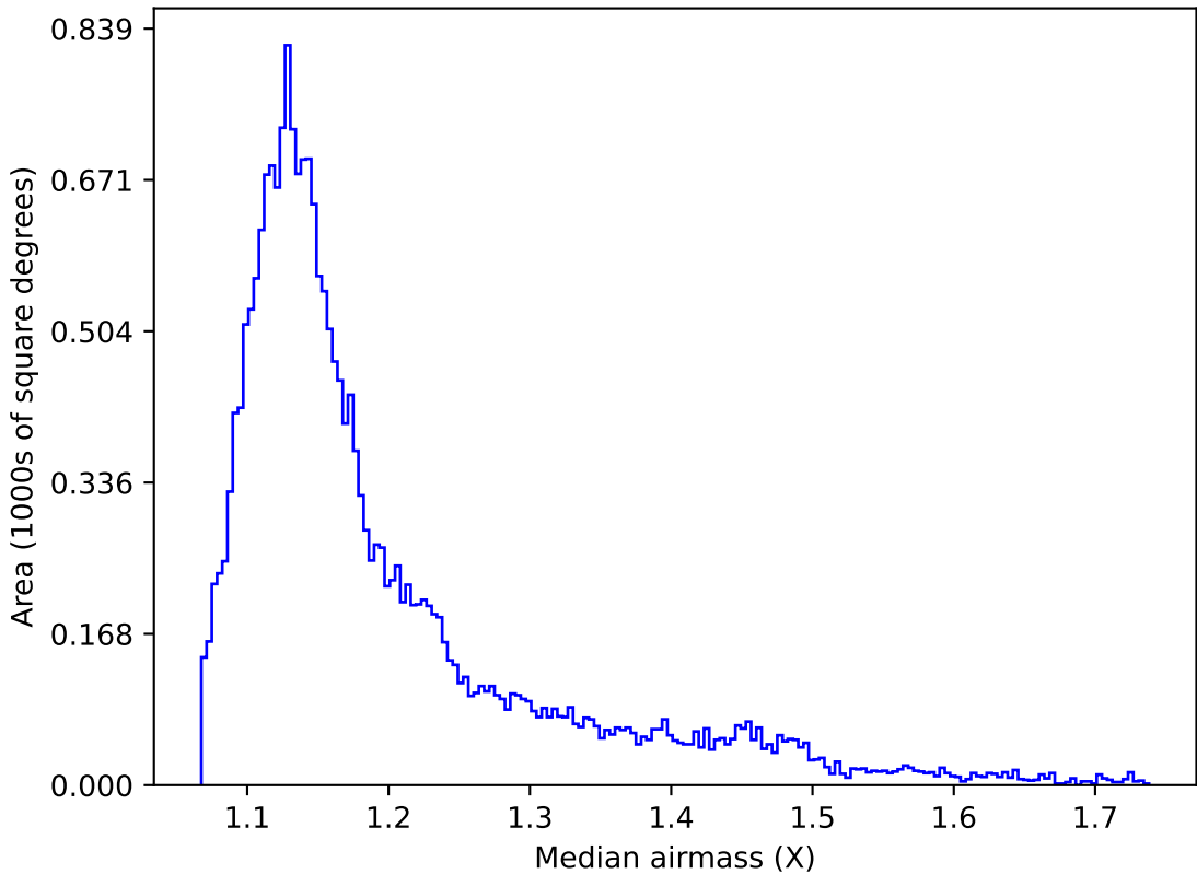
weather_cloudso1v3.4_10yrs All sky u band: Median airmass
