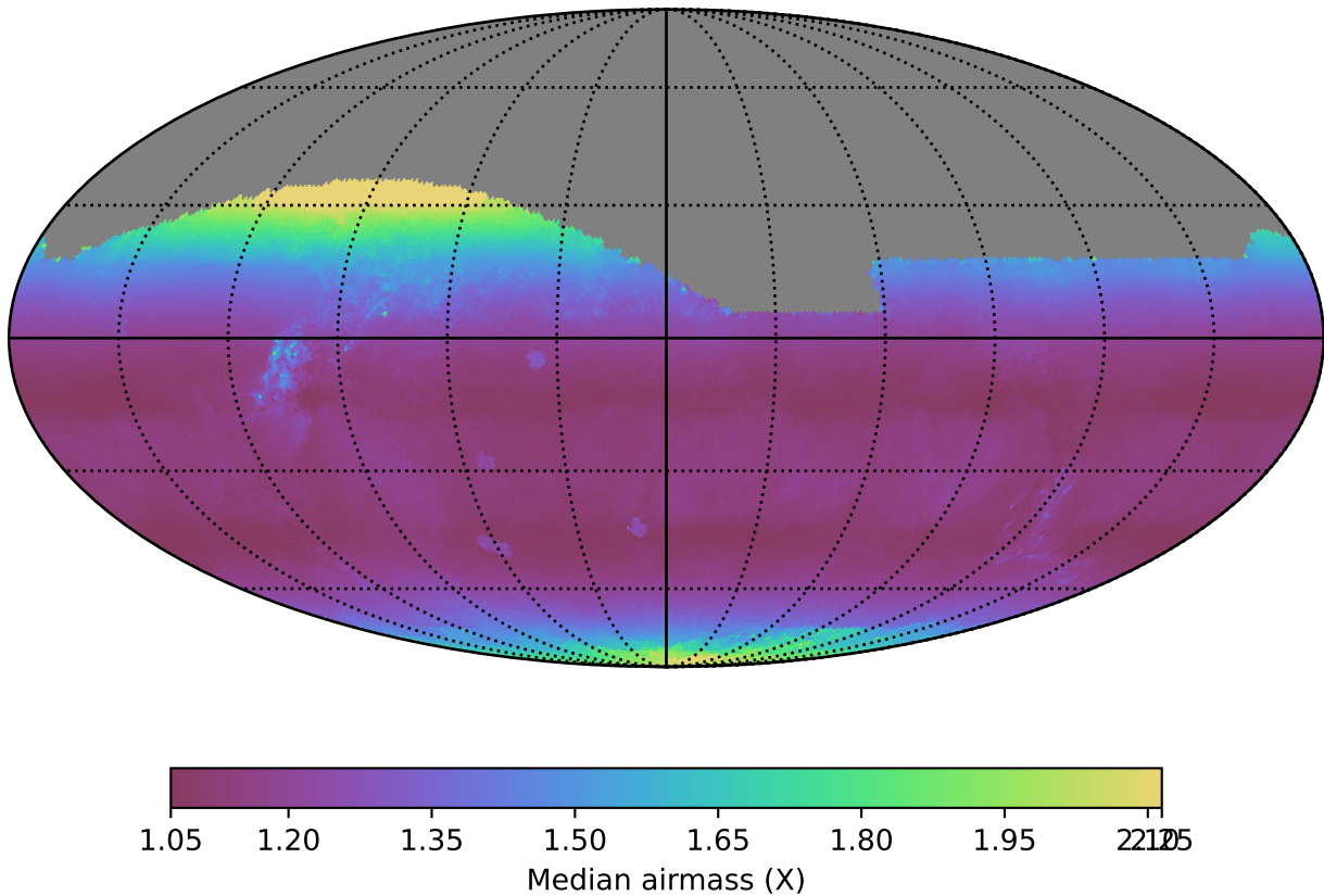
weather_cloudso1v3.4_10yrs All sky r band: Median airmass
