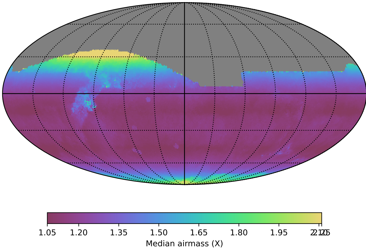
weather_cloudso1v3.4_10yrs All sky i band: Median airmass
