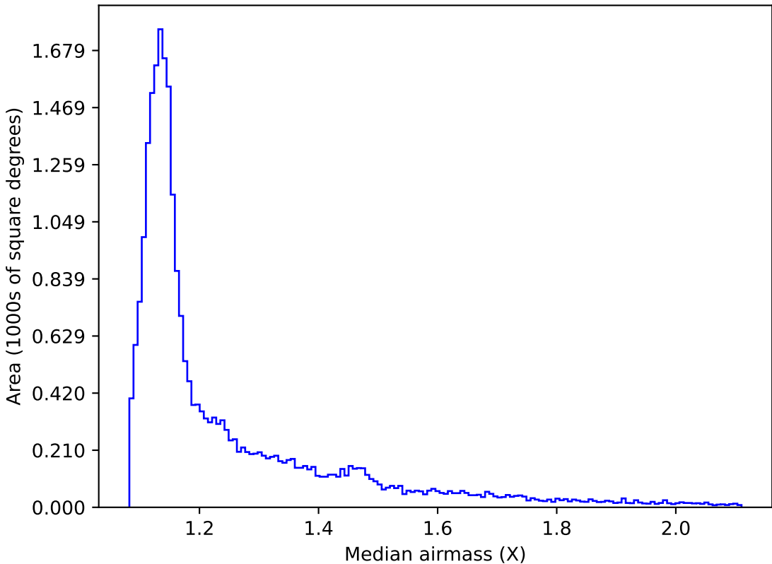
weather_cloudso1v3.4_10yrs All sky i band: Median airmass
