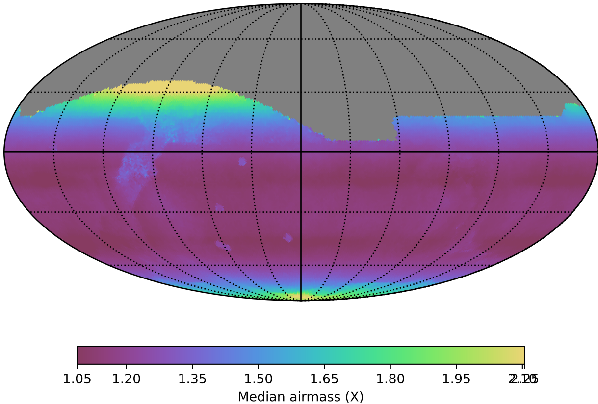
weather_cloudso1v3.4_10yrs All sky all bands: Median airmass
