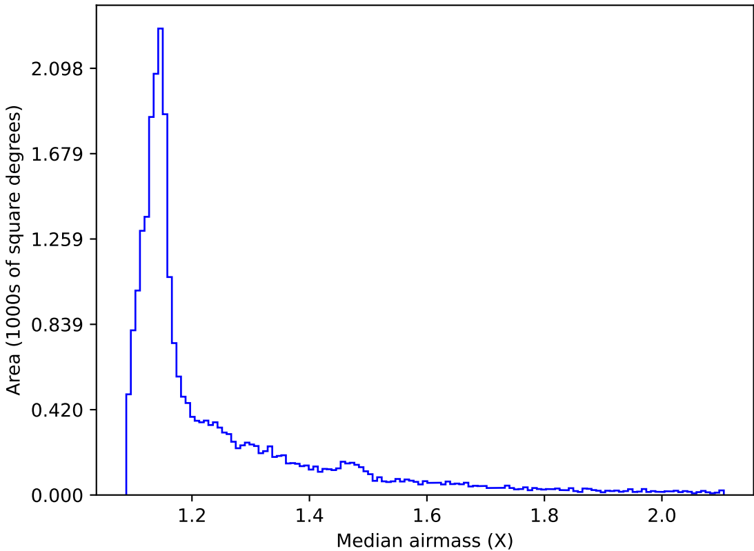
weather_cloudso1v3.4_10yrs All sky all bands: Median airmass
