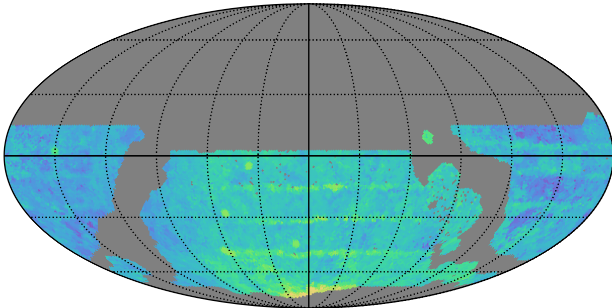
weather_cloudso1v3.4_10yrs WFD z band: Median Season Length
