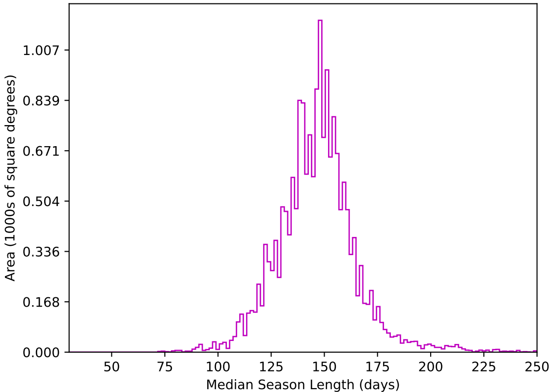
weather_cloudso1v3.4_10yrs WFD z band: Median Season Length
