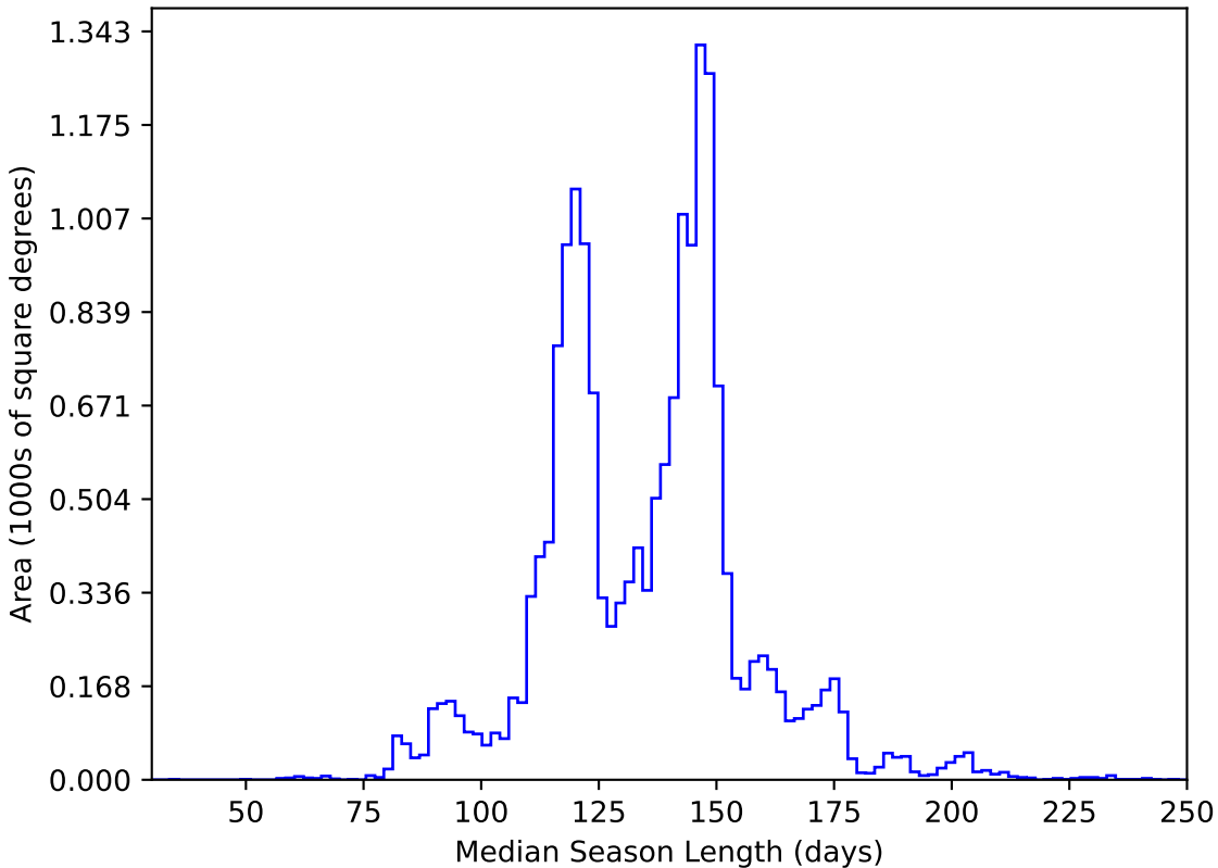
weather_cloudso1v3.4_10yrs WFD y band: Median Season Length
