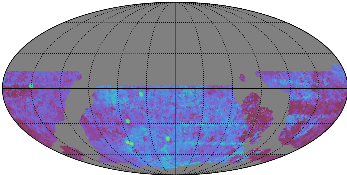
weather_cloudso1v3.4_10yrs WFD u band: Median Season Length
