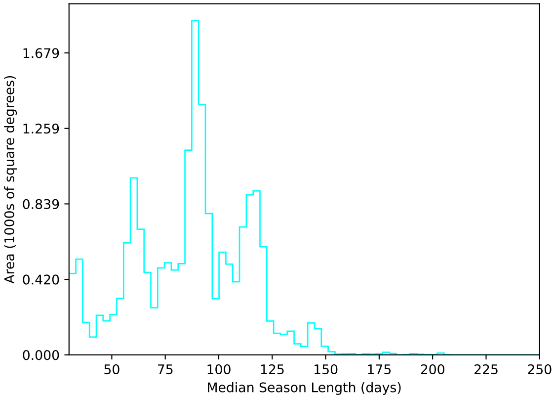
weather_cloudso1v3.4_10yrs WFD u band: Median Season Length
