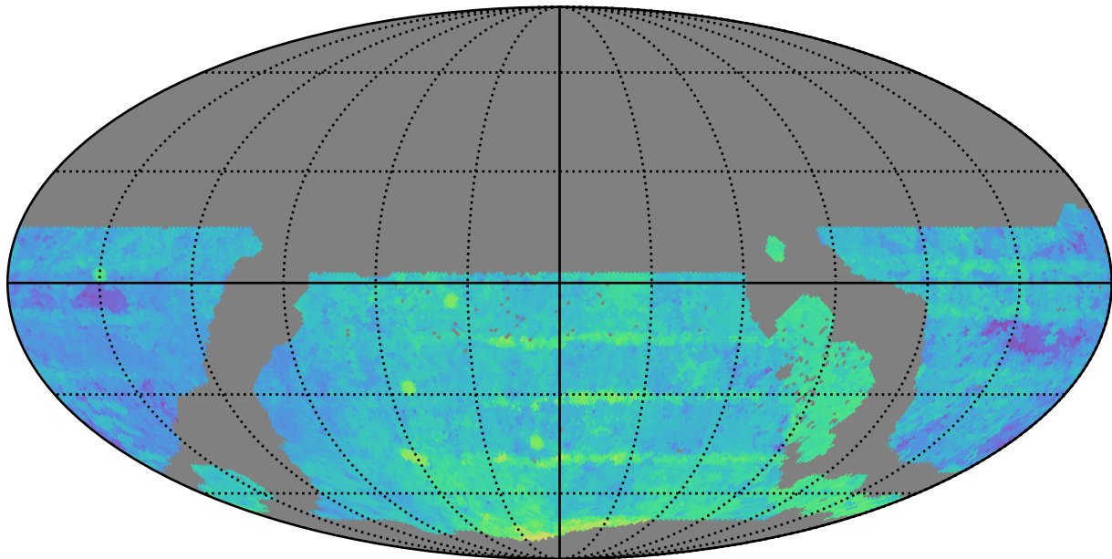
weather_cloudso1v3.4_10yrs WFD r band: Median Season Length
