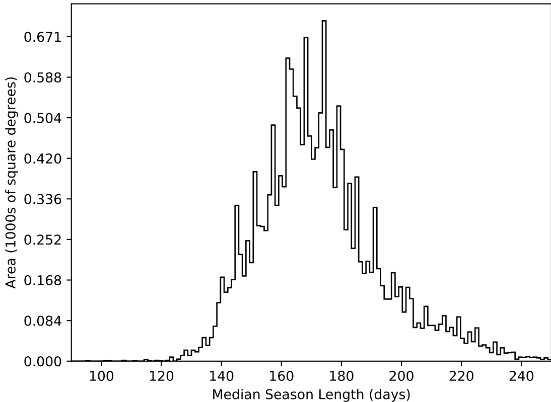
weather_cloudso1v3.4_10yrs WFD all bands: Median Season Length
