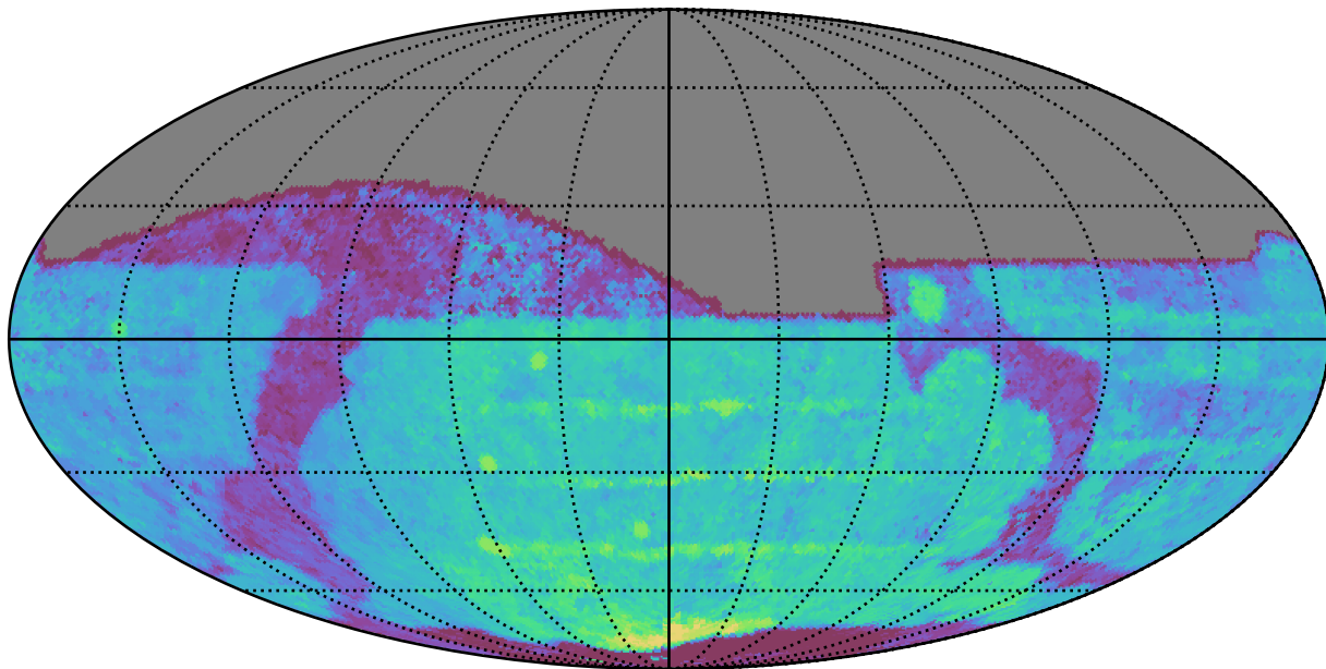
weather_cloudso1v3.4_10yrs All sky z band: Median Season Length
