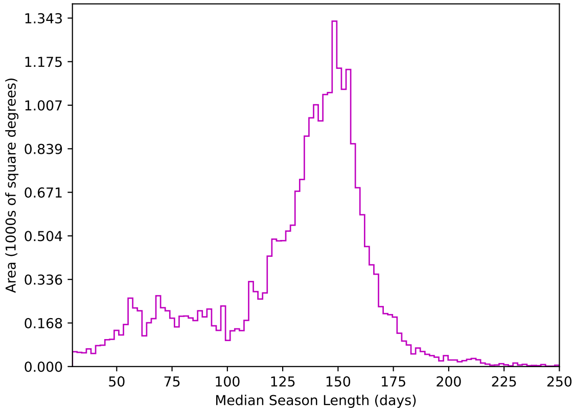
weather_cloudso1v3.4_10yrs All sky z band: Median Season Length
