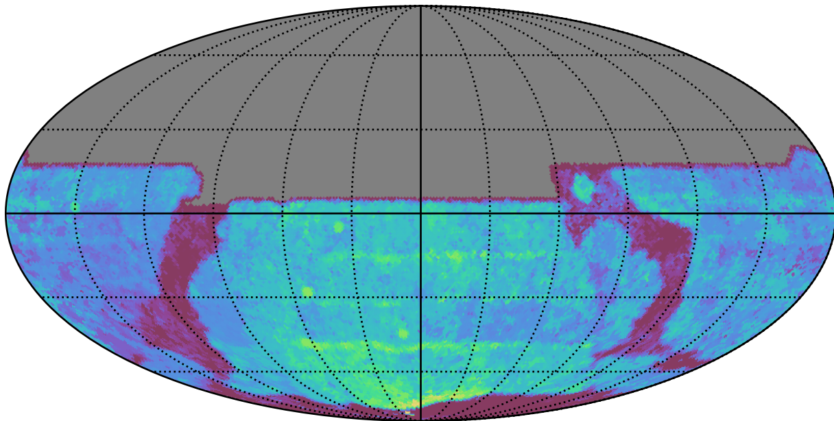
weather_cloudso1v3.4_10yrs All sky y band: Median Season Length
