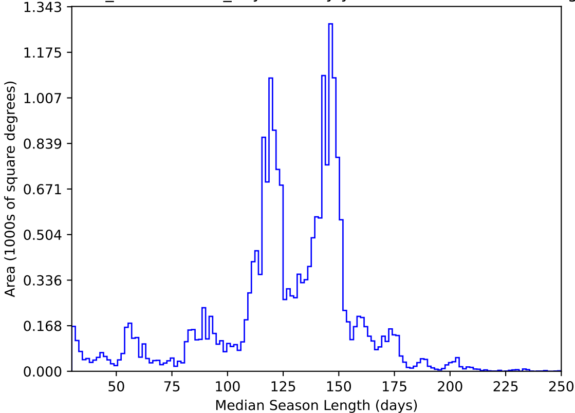
weather_cloudso1v3.4_10yrs All sky y band: Median Season Length
