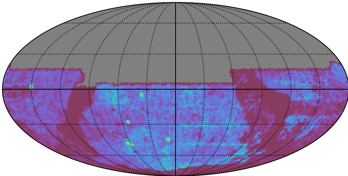
weather_cloudso1v3.4_10yrs All sky u band: Median Season Length
