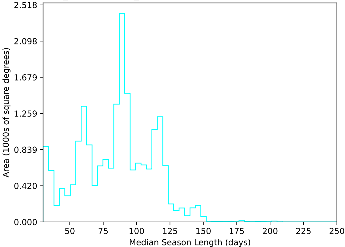
weather_cloudso1v3.4_10yrs All sky u band: Median Season Length
