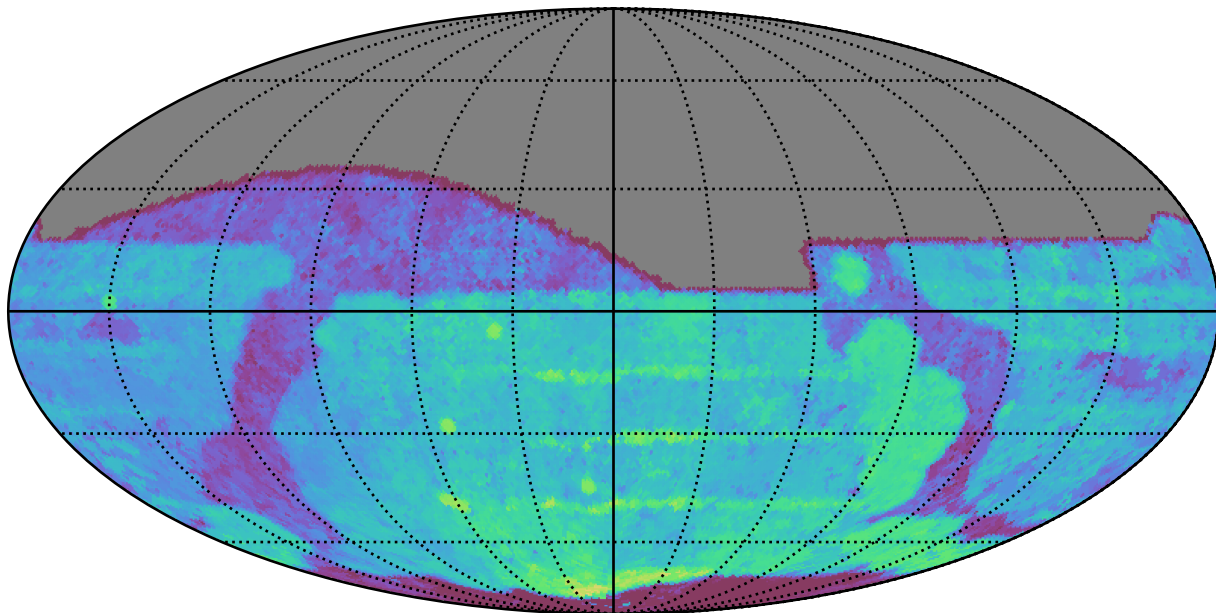
weather_cloudso1v3.4_10yrs All sky r band: Median Season Length
