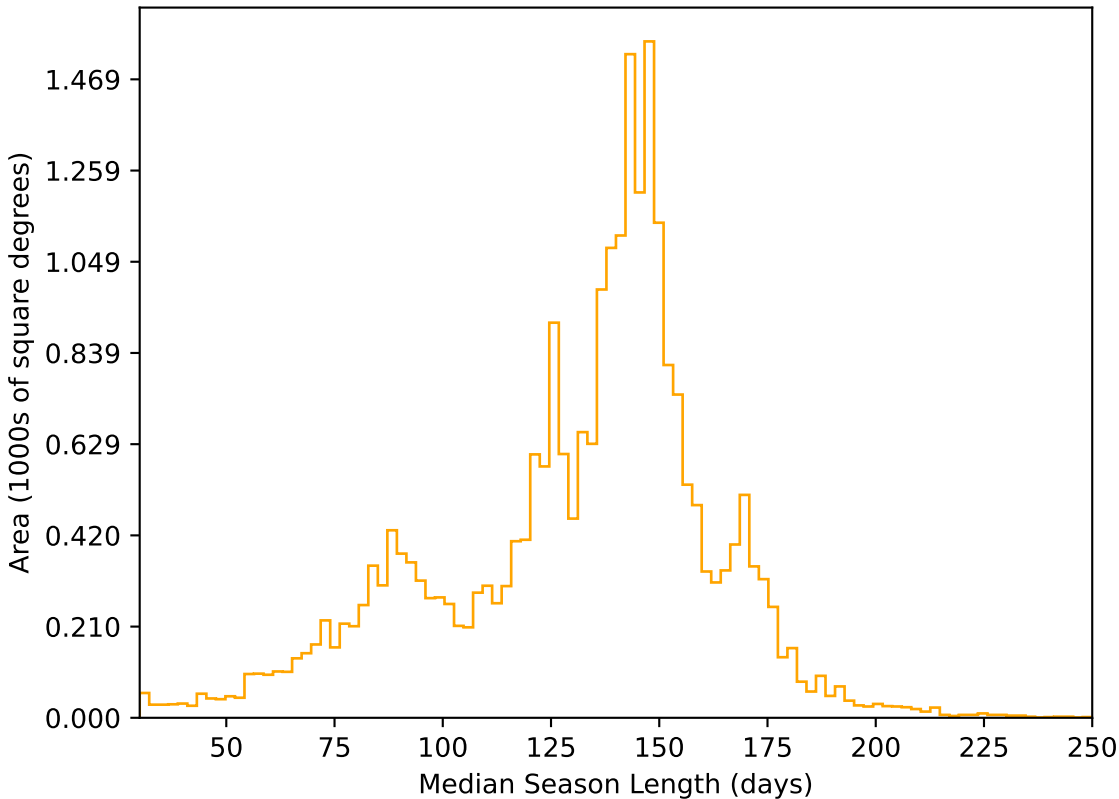
weather_cloudso1v3.4_10yrs All sky r band: Median Season Length
