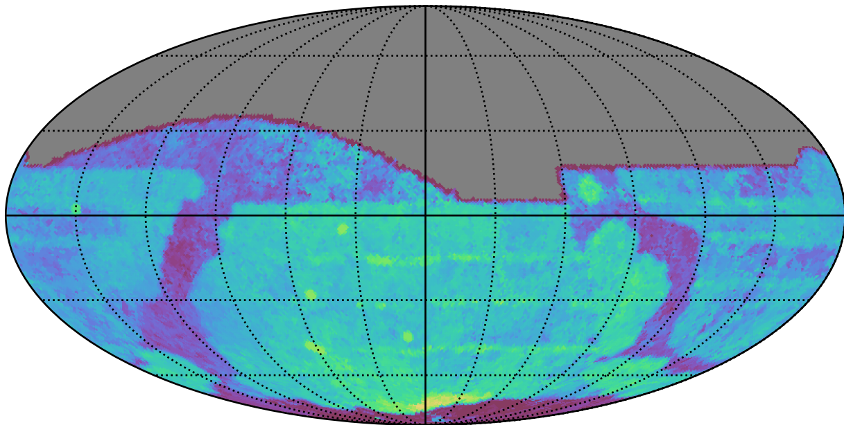
weather_cloudso1v3.4_10yrs All sky i band: Median Season Length
