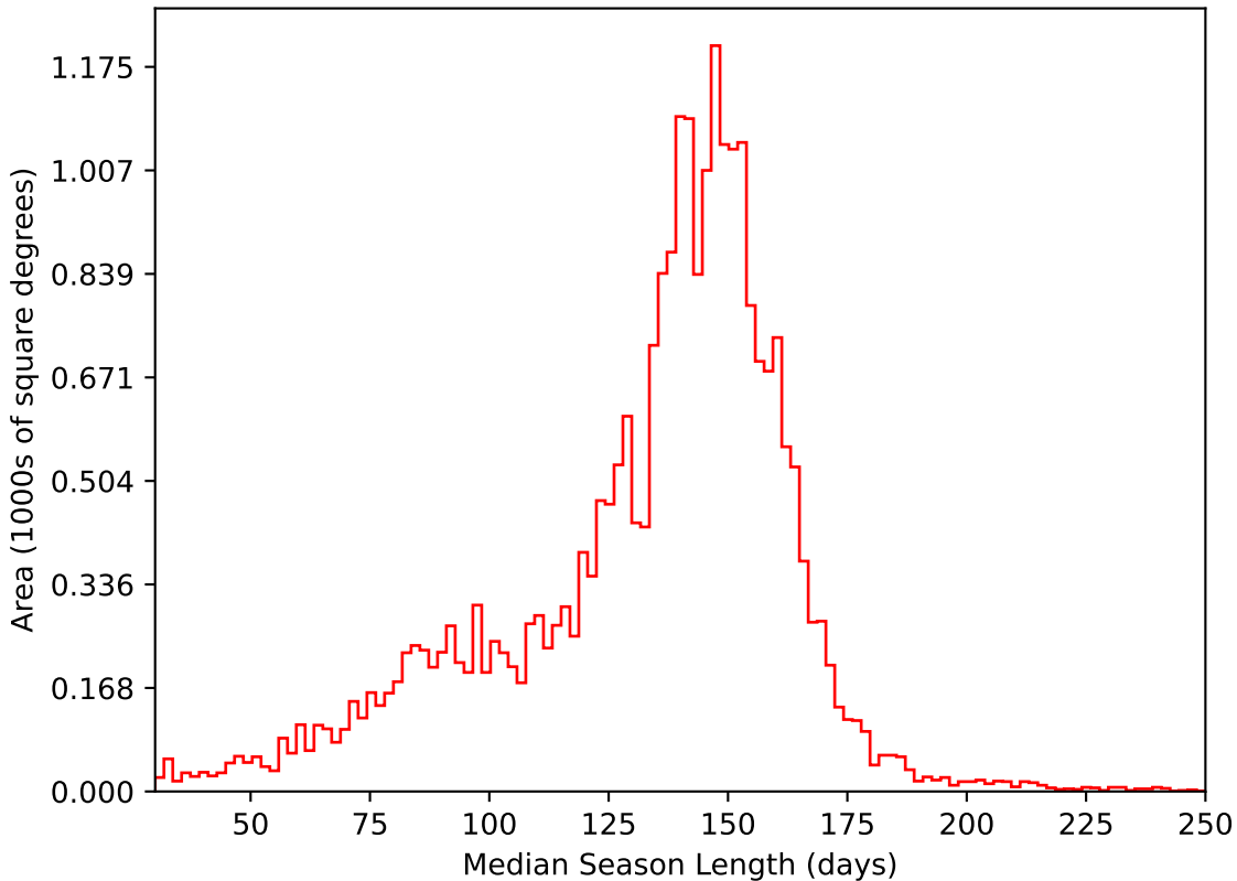
weather_cloudso1v3.4_10yrs All sky i band: Median Season Length
