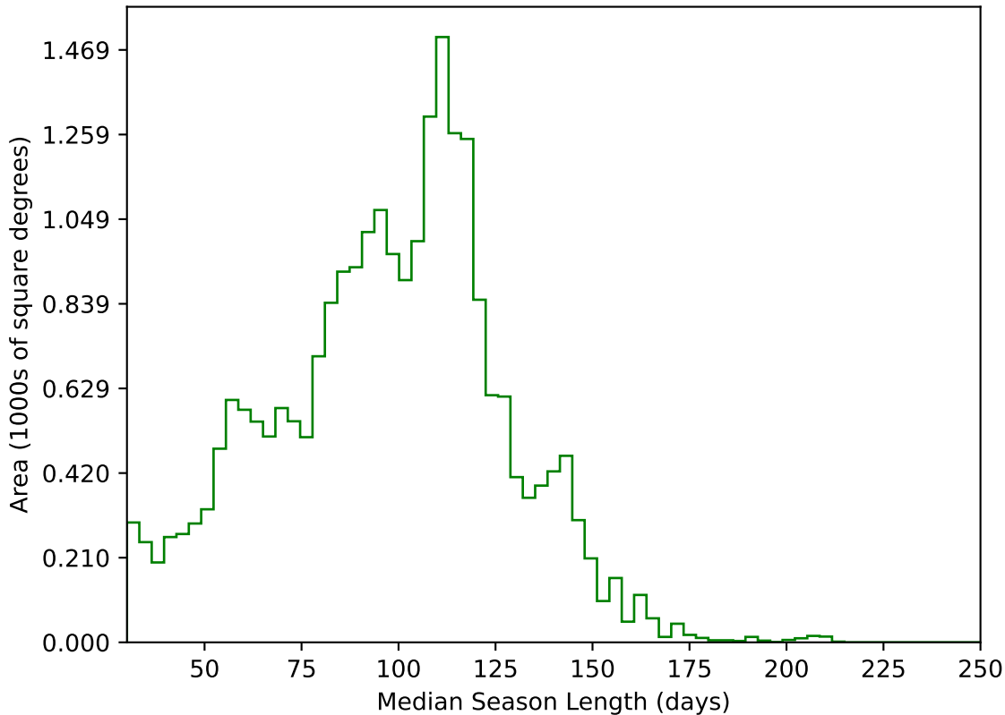
weather_cloudso1v3.4_10yrs All sky g band: Median Season Length
