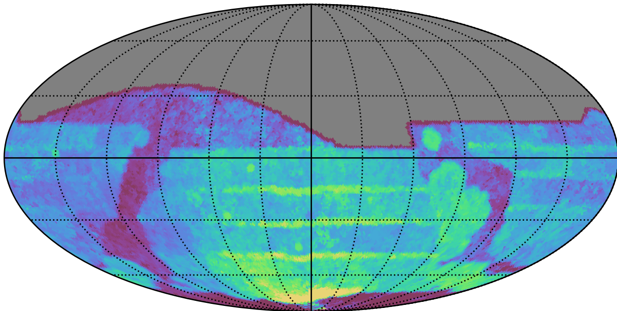
weather_cloudso1v3.4_10yrs All sky all bands: Median Season Length
