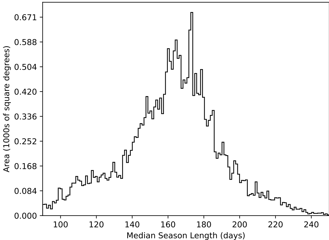
weather_cloudso1v3.4_10yrs All sky all bands: Median Season Length
