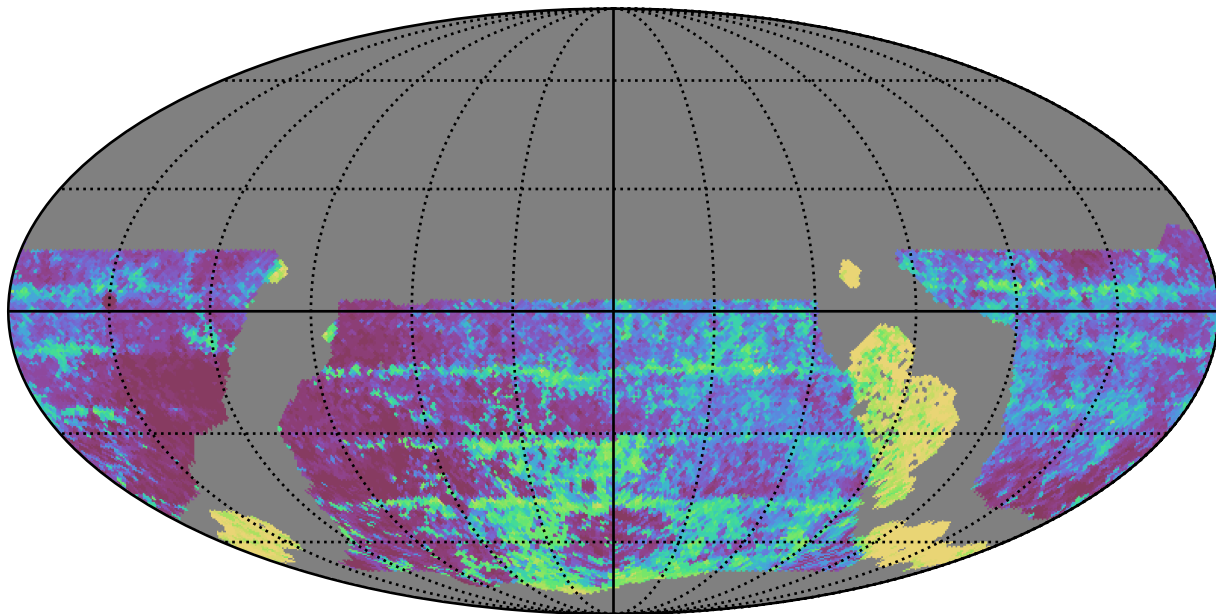
weather_cloudso1v3.4_10yrs WFD y band: Median Inter-Night Gap
