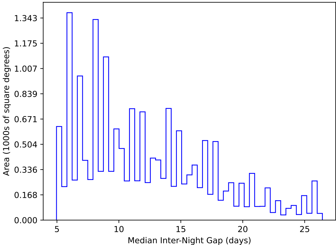
weather_cloudso1v3.4_10yrs WFD y band: Median Inter-Night Gap
