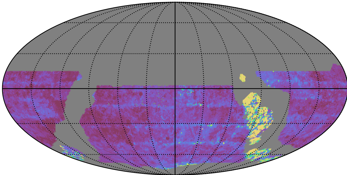
weather_cloudso1v3.4_10yrs WFD u band: Median Inter-Night Gap
