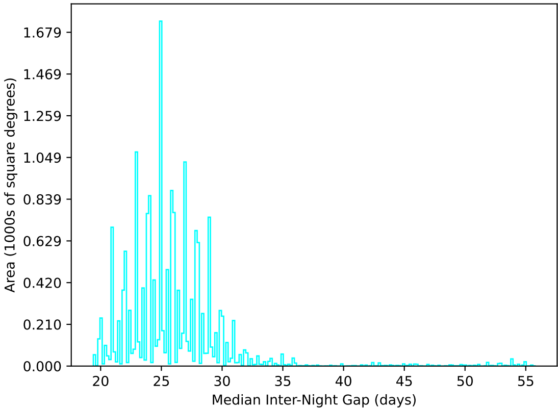
weather_cloudso1v3.4_10yrs WFD u band: Median Inter-Night Gap
