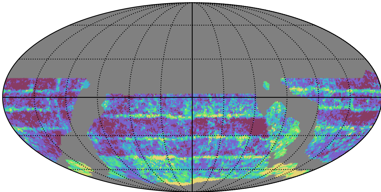
weather_cloudso1v3.4_10yrs WFD r band: Median Inter-Night Gap
