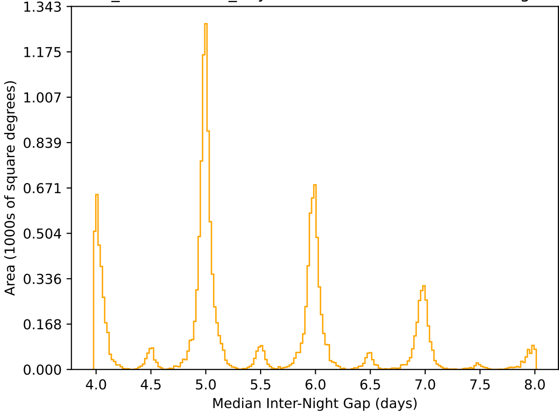
weather_cloudso1v3.4_10yrs WFD r band: Median Inter-Night Gap
