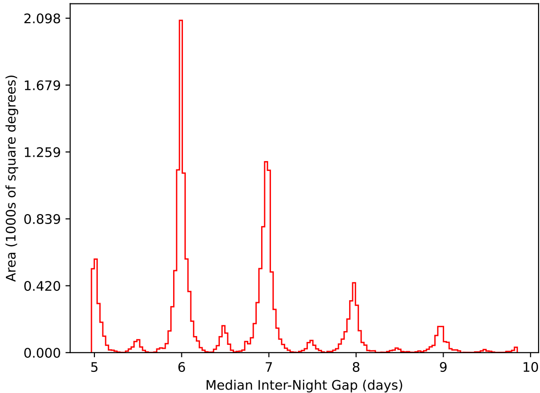
weather_cloudso1v3.4_10yrs WFD i band: Median Inter-Night Gap
