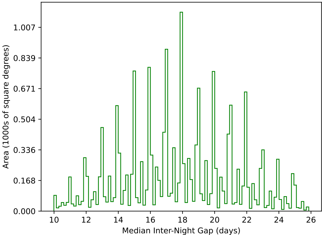
weather_cloudso1v3.4_10yrs WFD g band: Median Inter-Night Gap
