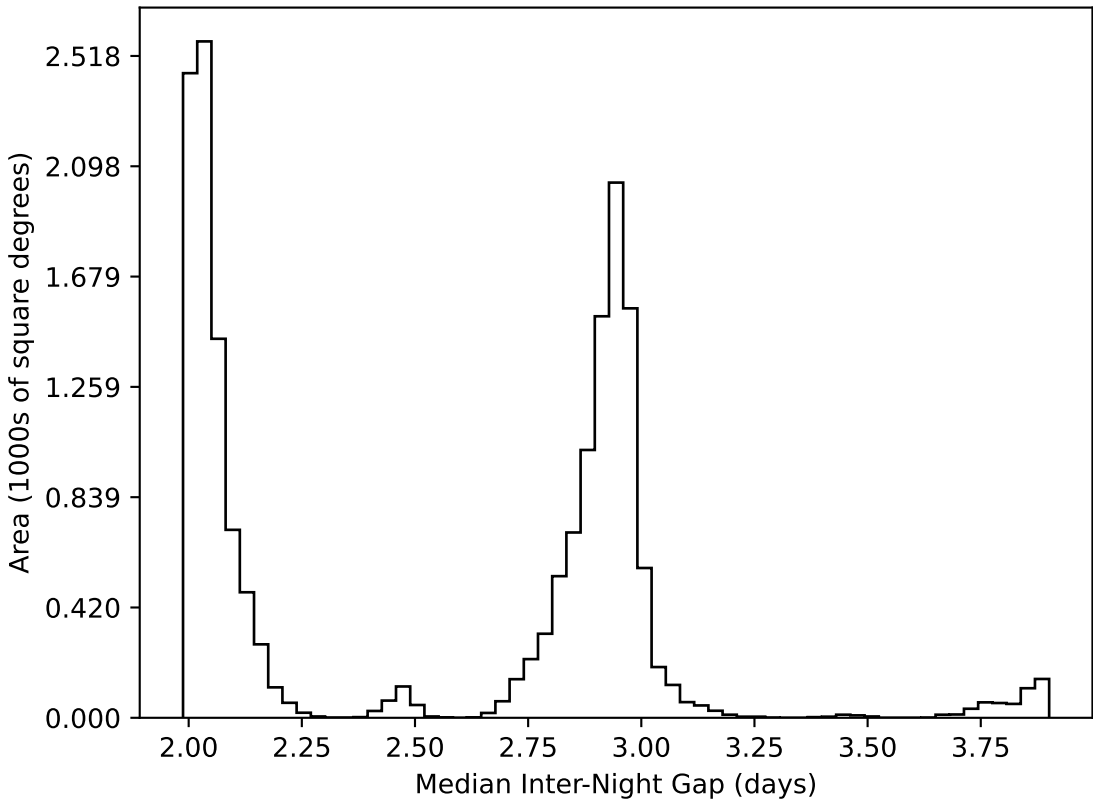
weather_cloudso1v3.4_10yrs WFD all bands: Median Inter-Night Gap
