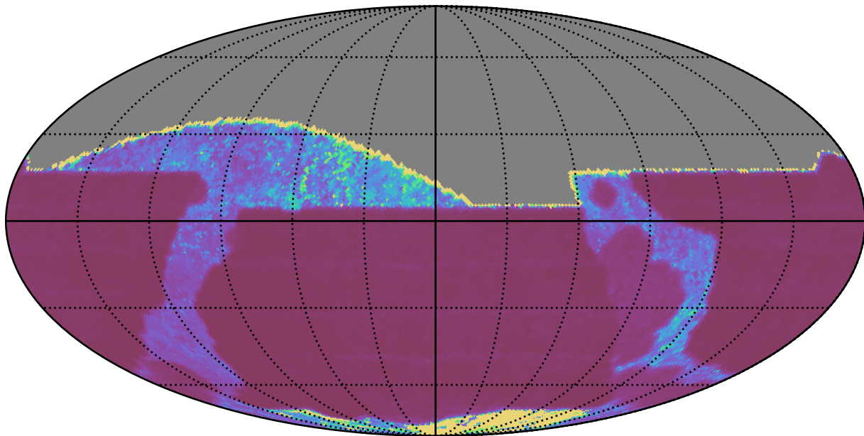
weather_cloudso1v3.4_10yrs All sky z band: Median Inter-Night Gap
