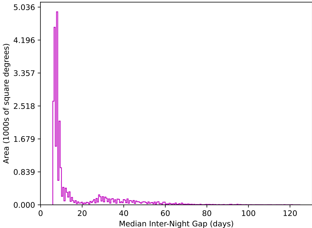
weather_cloudso1v3.4_10yrs All sky z band: Median Inter-Night Gap
