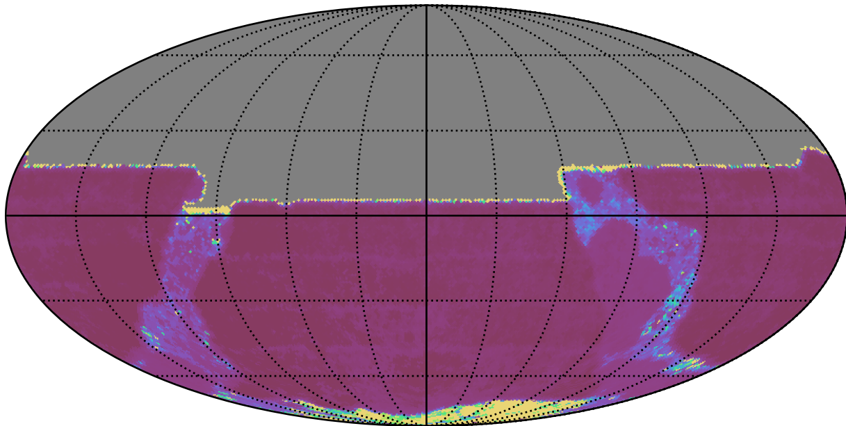
weather_cloudso1v3.4_10yrs All sky y band: Median Inter-Night Gap
