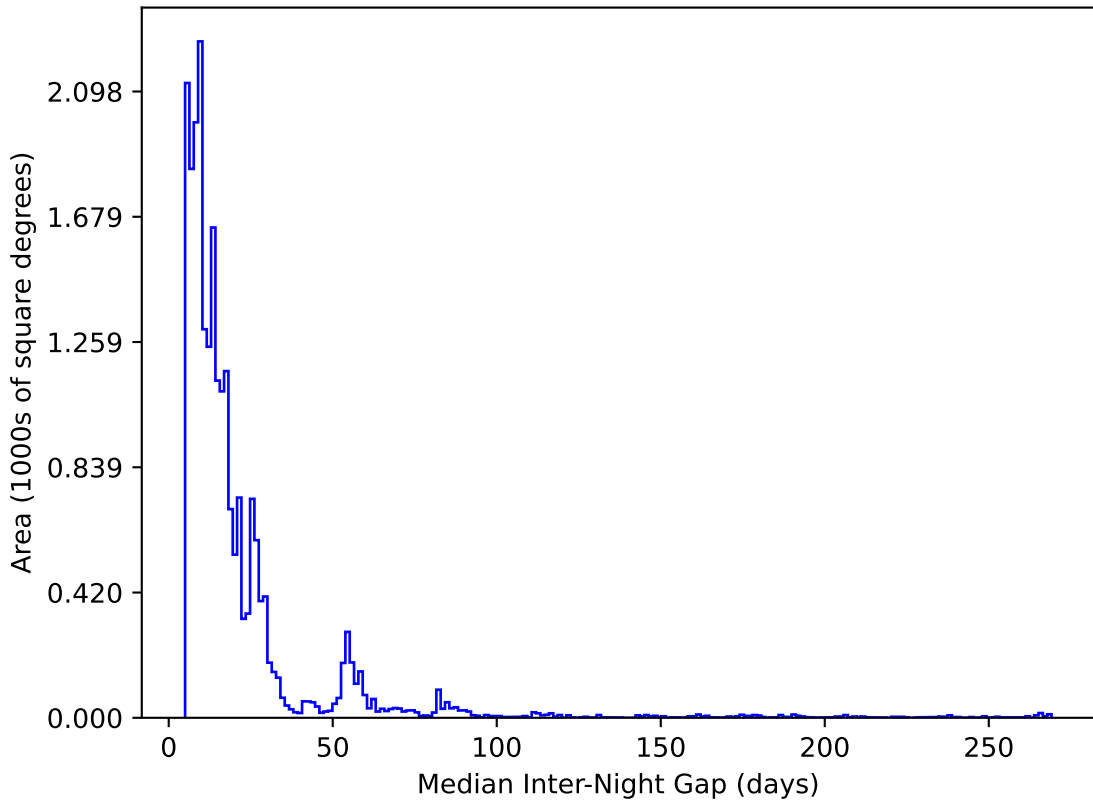
weather_cloudso1v3.4_10yrs All sky y band: Median Inter-Night Gap
