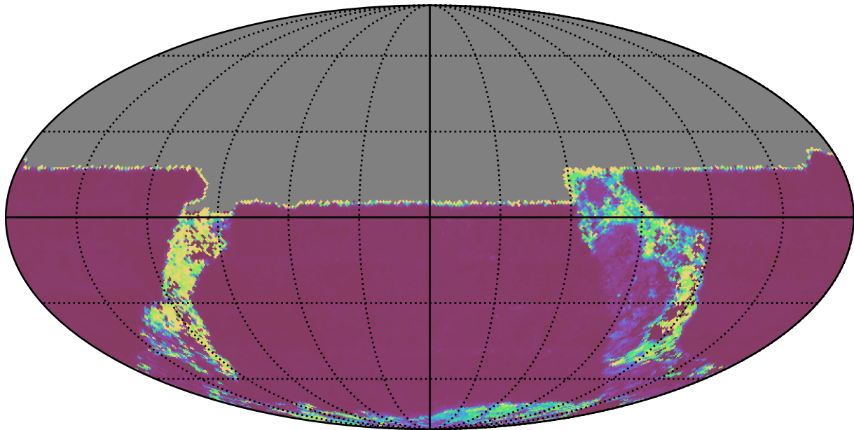
weather_cloudso1v3.4_10yrs All sky u band: Median Inter-Night Gap
