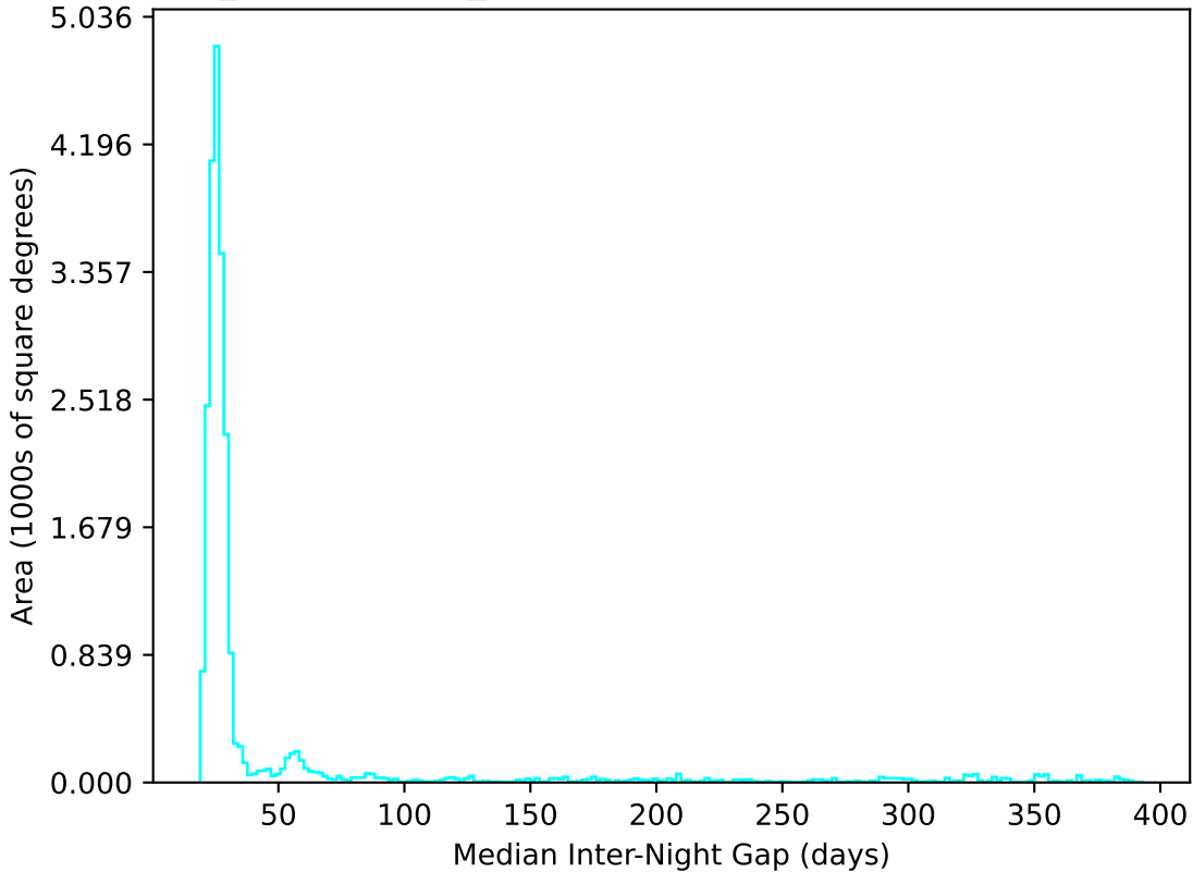
weather_cloudso1v3.4_10yrs All sky u band: Median Inter-Night Gap
