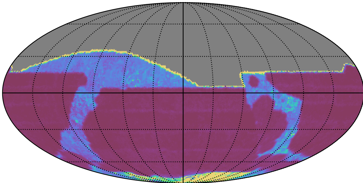
weather_cloudso1v3.4_10yrs All sky r band: Median Inter-Night Gap
