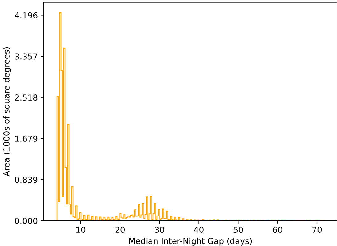
weather_cloudso1v3.4_10yrs All sky r band: Median Inter-Night Gap
