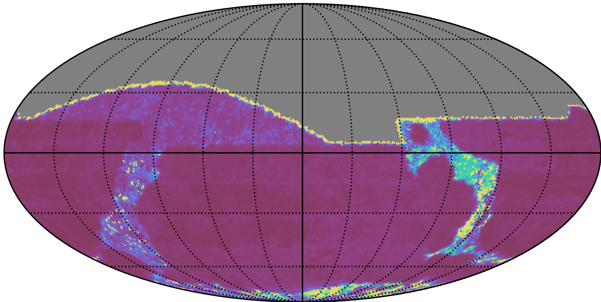
weather_cloudso1v3.4_10yrs All sky g band: Median Inter-Night Gap
