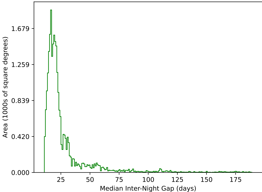
weather_cloudso1v3.4_10yrs All sky g band: Median Inter-Night Gap
