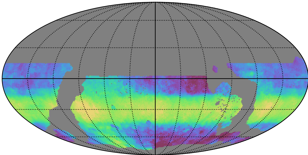
weather_cloudso1v3.4_10yrs WFD z band: Median HA
