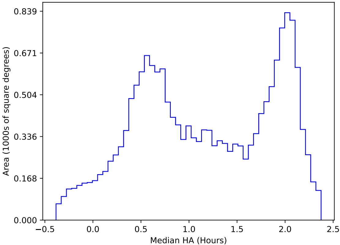
weather_cloudso1v3.4_10yrs WFD z band: Median HA
